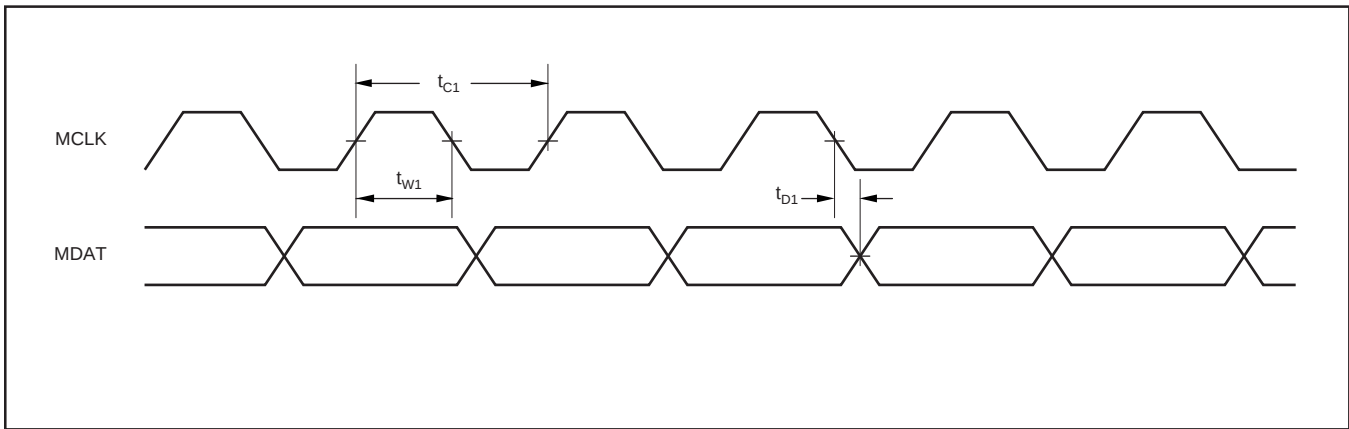
DIAGRAM 1: Mode 0 Operation.
