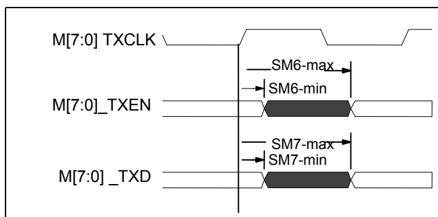
Figure 15 - AC Characteristics – General Purpose Serial Interface (TX)
