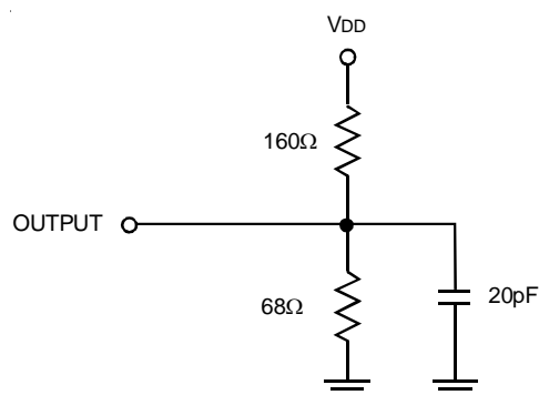
TEST CIRCUIT 1
