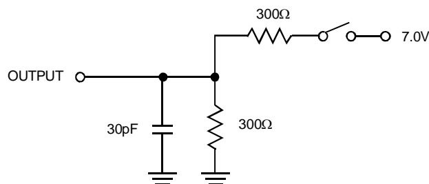
TEST CIRCUIT 2
