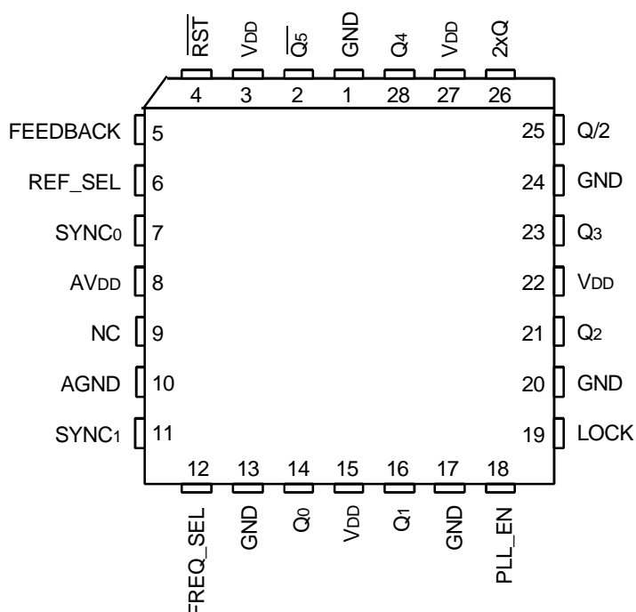
PLCC TOP VIEW
