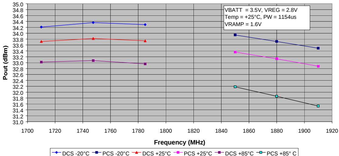
Figure 6: DCS/PCS P MAX vs. Temperature @ V ramp = V rampmax = 1.6V (2TX slots)
