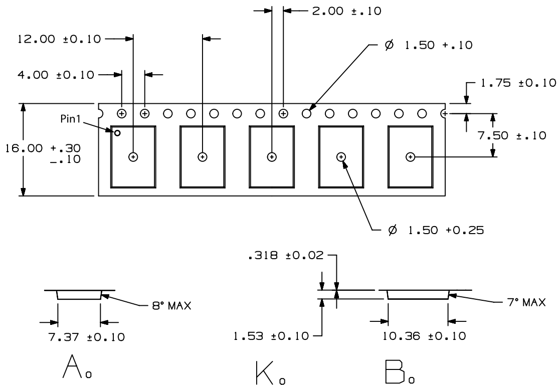
Figure 9: Tape &amp; Reel Packaging
