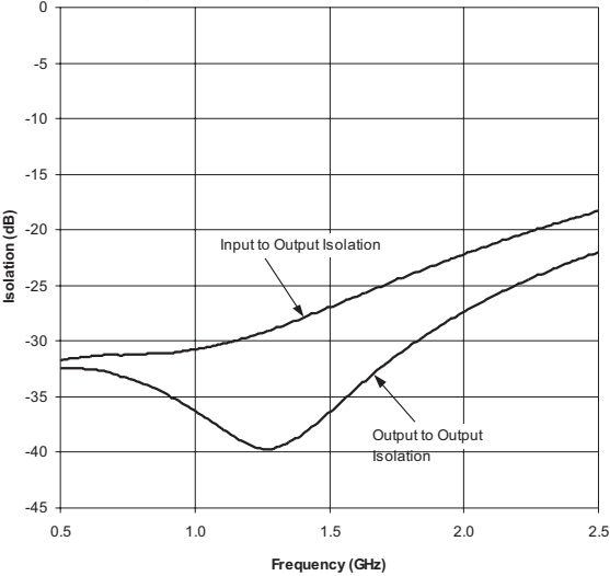
Figure 3: Isolation vs. Frequency
