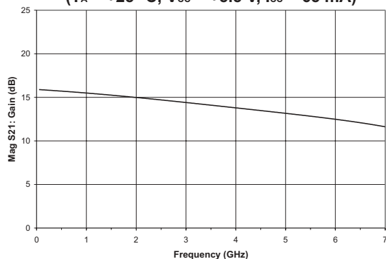
Figure 4: Gain vs. Frequency De-embedded 50 \Omega S-parameter ( T_A = +25^\circ\text{C} , V_{CC} = +5.5\text{ V} , I_{CC} = 65\text{ mA} )
