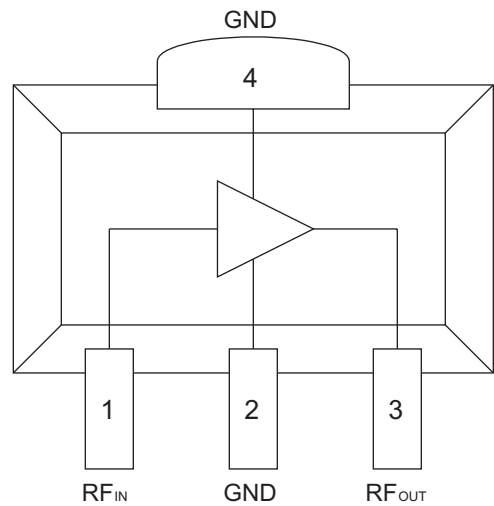
Figure 2: Pinout (X-ray Top View)
