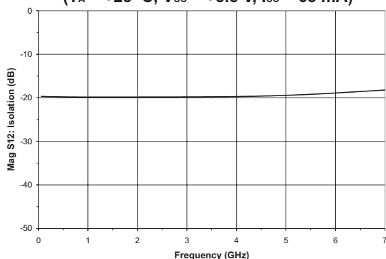
Figure 5: Isolation vs. Frequency De-embedded 50 \Omega S-parameter ( T_A = +25^\circ\text{C} , V_{CC} = +5.5\text{ V} , I_{CC} = 65\text{ mA} )
