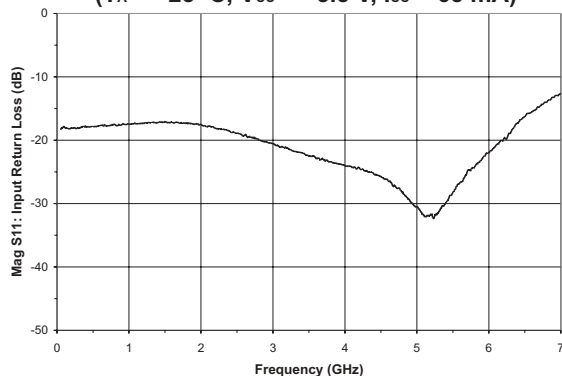
Figure 6: Input Return Loss vs. Frequency De-embedded 50 \Omega S-parameter ( T_A = +25^\circ\text{C} , V_{CC} = +5.5\text{ V} , I_{CC} = 65\text{ mA} )
