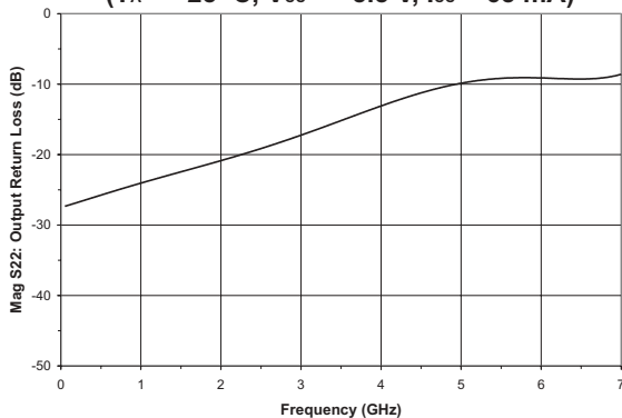
Figure 7: Output Return Loss vs. Frequency De-embedded 50 \Omega S-parameter ( T_A = +25^\circ\text{C} , V_{CC} = +5.5\text{ V} , I_{CC} = 65\text{ mA} )
