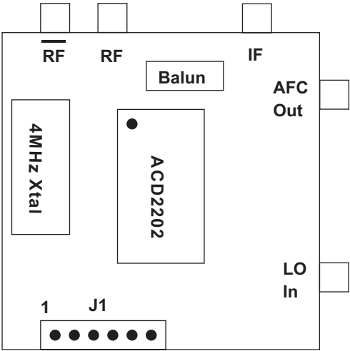
Figure 26: Evaluation Fixture
