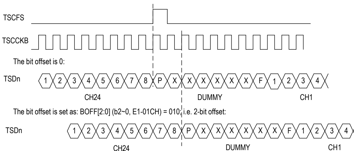
Figure - 61. Transmit Bit Offset in T1/J1 Mode - 1
