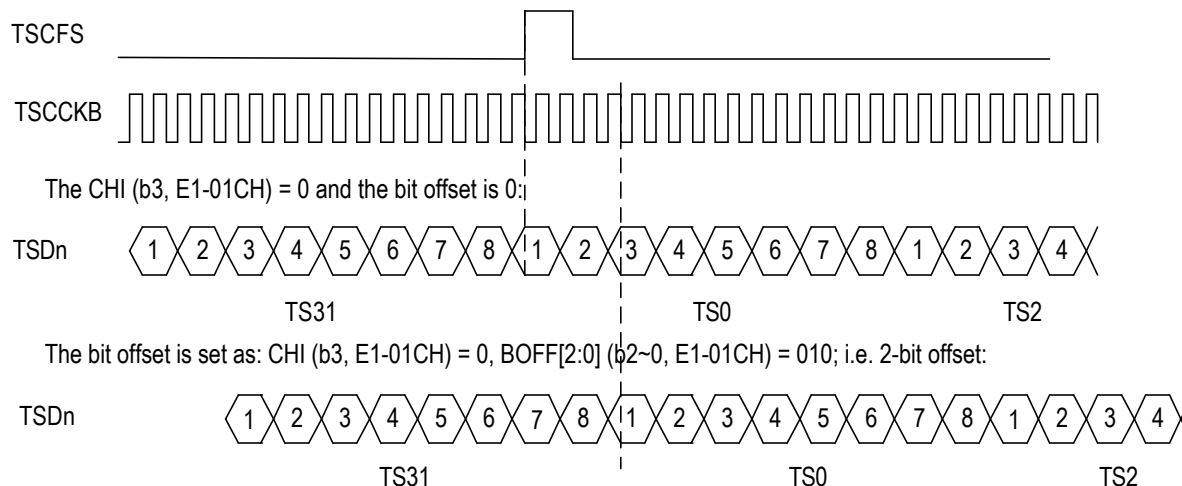
Figure - 47. Transmit Bit Offset in E1 Mode - 2
