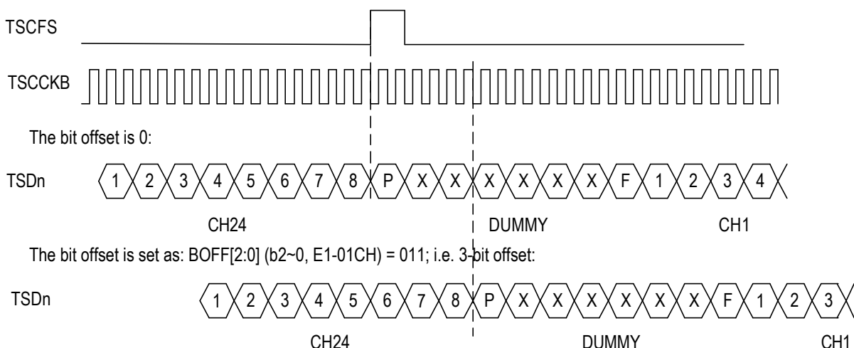
Figure - 62. Transmit Bit Offset in T1/J1 Mode - 2
