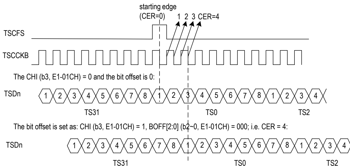
Figure - 48. Transmit Bit Offset in E1 Mode - 3
