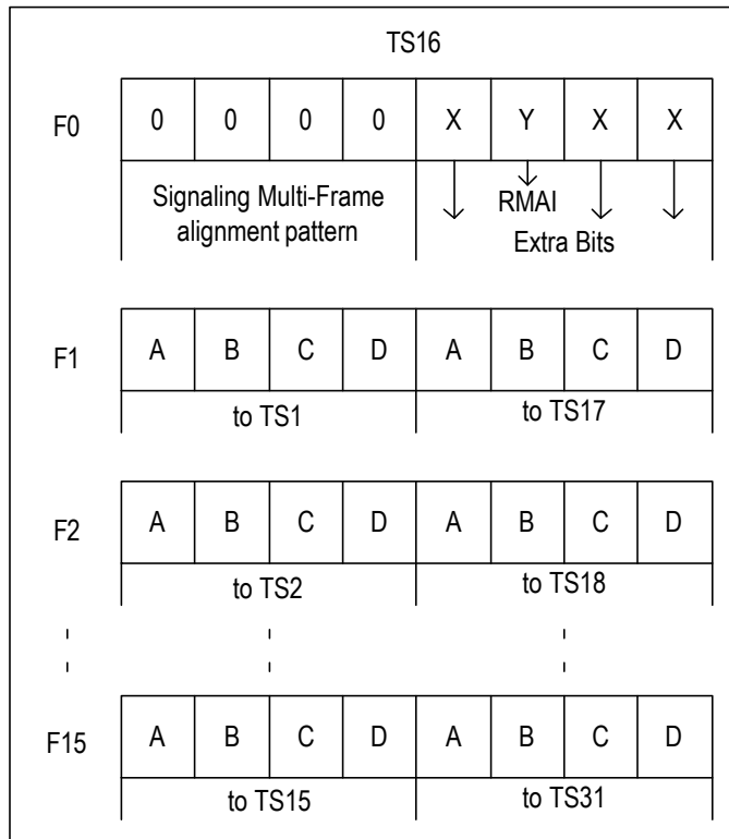
Figure - 4. TS16 Arrangement in Signaling Multi-Frame
