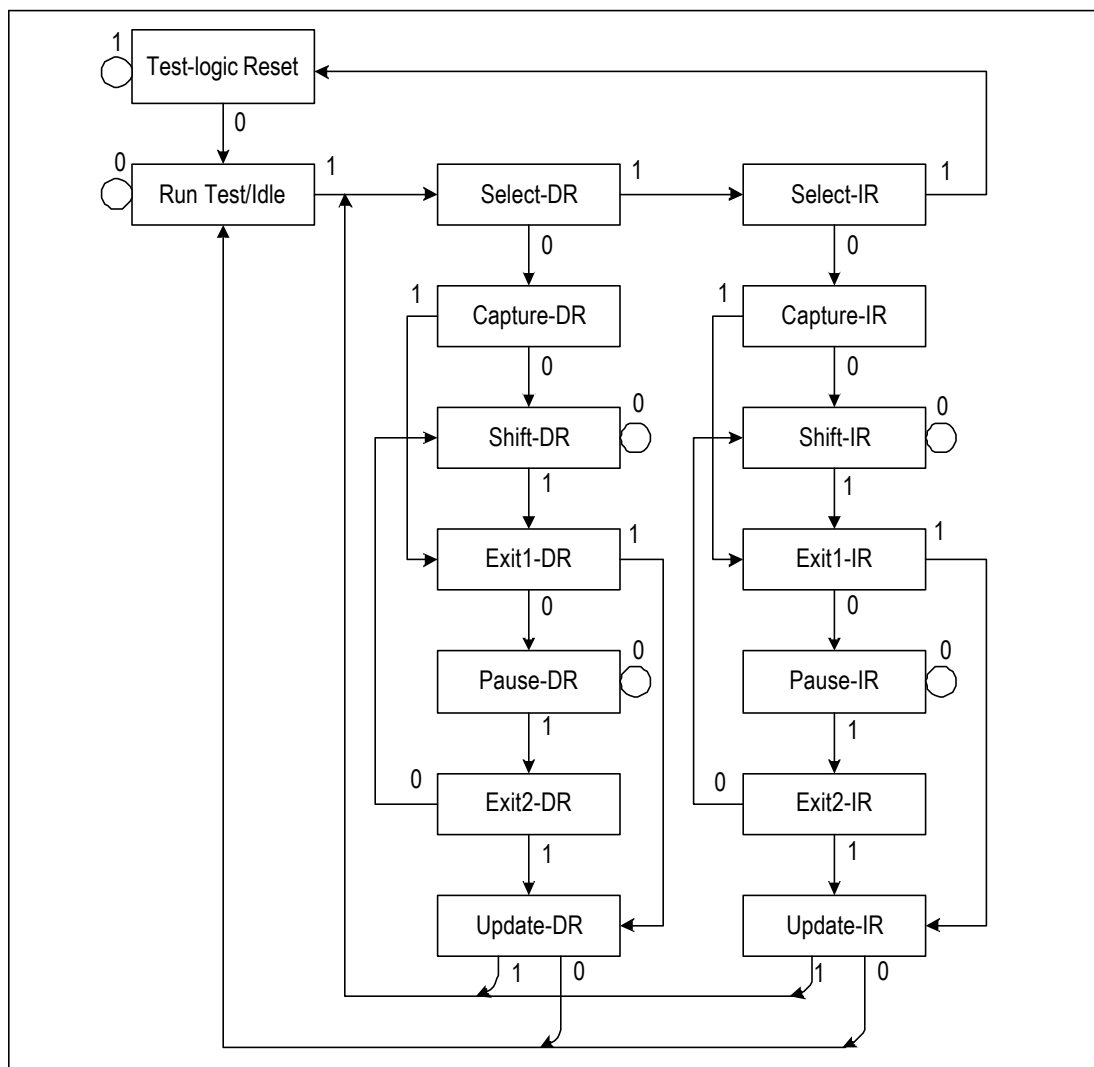
Figure - 84. JTAG State Diagram
