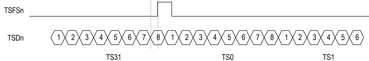
Figure - 42. E1 Transmit Clock Master Mode - Functional Timing Example
