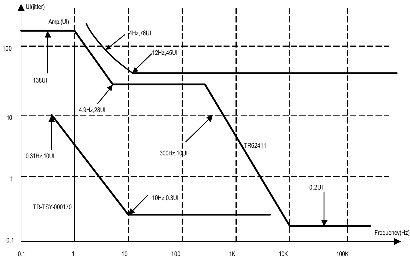
Figure - 65. T1/J1 Mode Jitter Tolerance ( N1 = N2 = 2fH )
