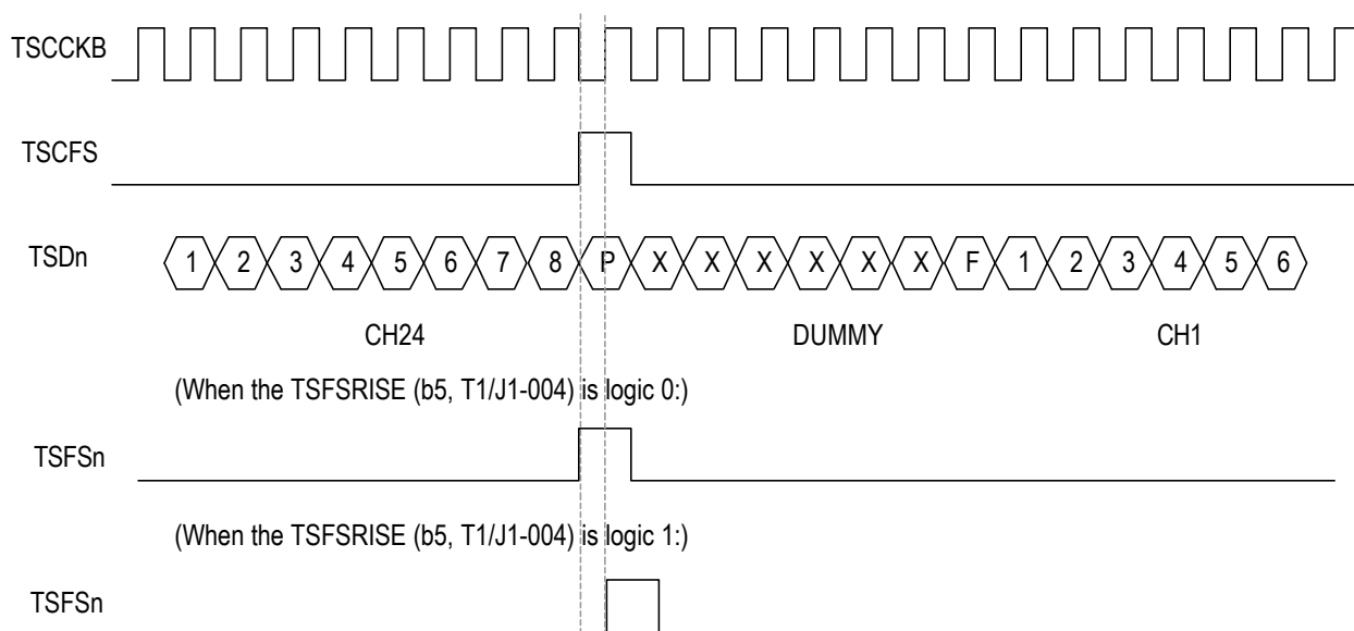
Figure - 53. T1/J1 Transmit Clock Slave TSFS Enable Mode - Functional Timing Example 2
