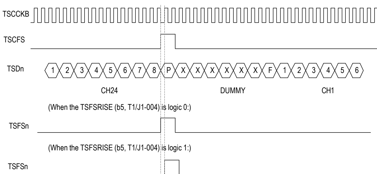
Figure - 54. T1/J1 Transmit Clock Slave TSFS Enable Mode - Functional Timing Example 3
