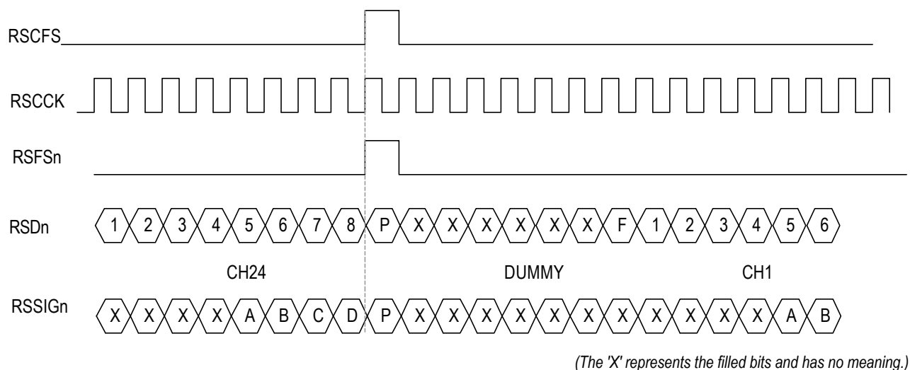
Figure - 27. T1/J1 Receive Clock Slave External Signaling Mode - Functional Timing Example 2
