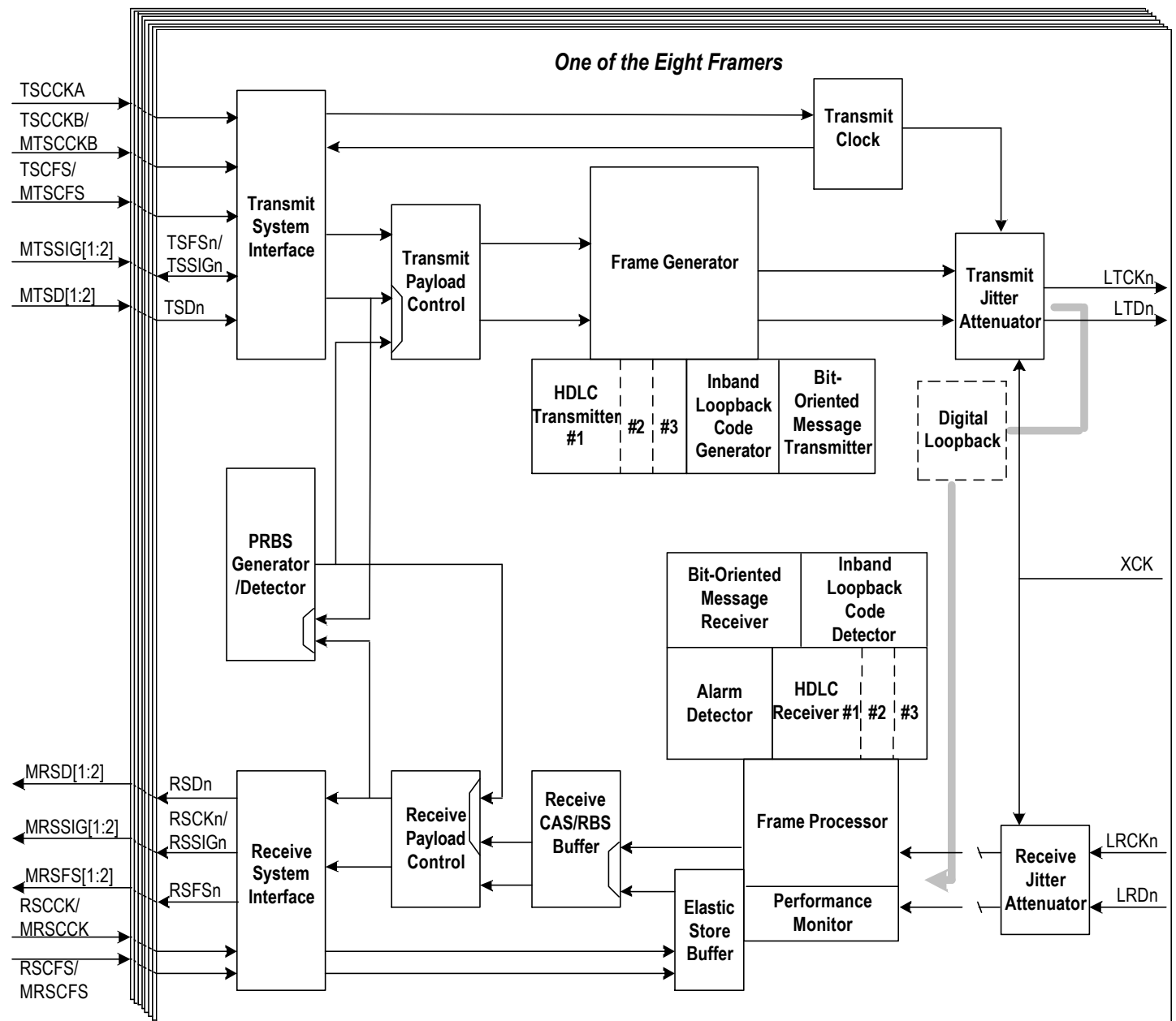
Figure - 69. Digital Loopback
