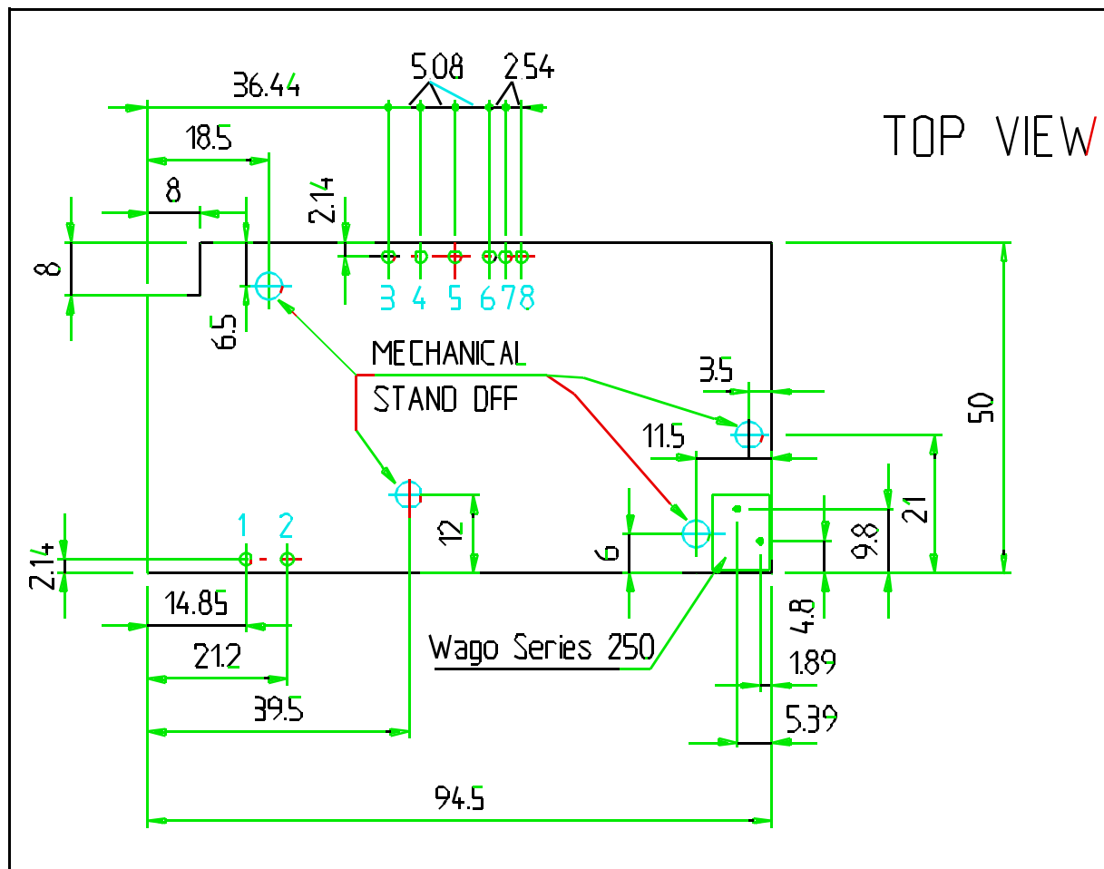
COMBI/E1-I Power Management Module TOP VIEW (dimensions in mm)
