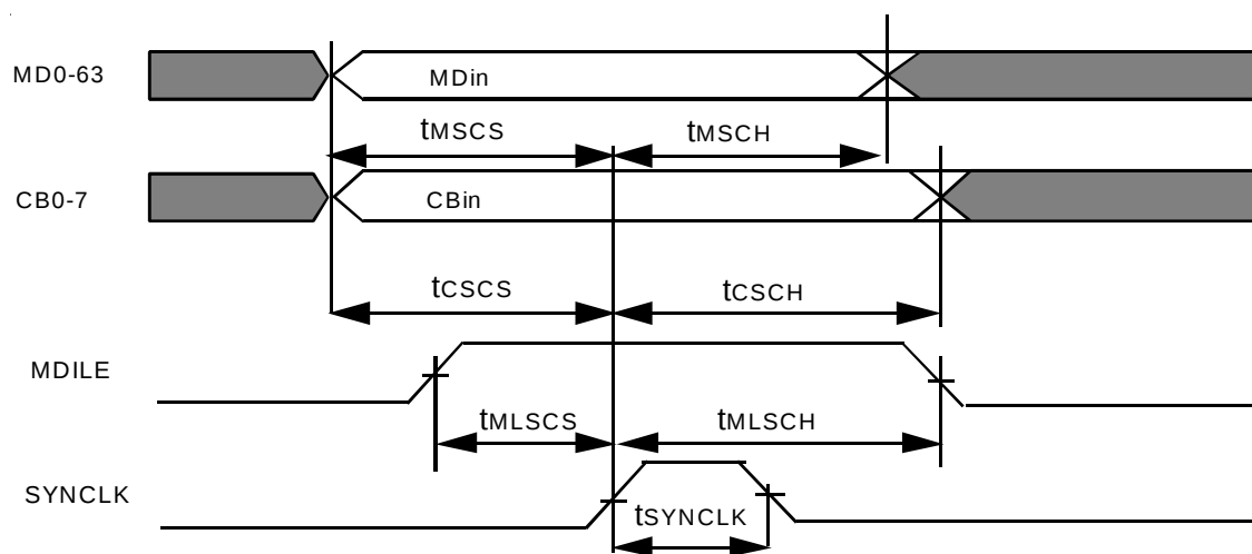
Figure 14. Diagnostic Timing
