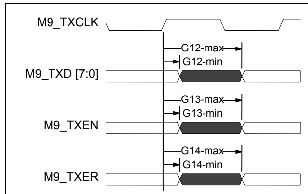
Figure 21 - AC Characteristics- Gigabit Media Independent Interface (TX)
