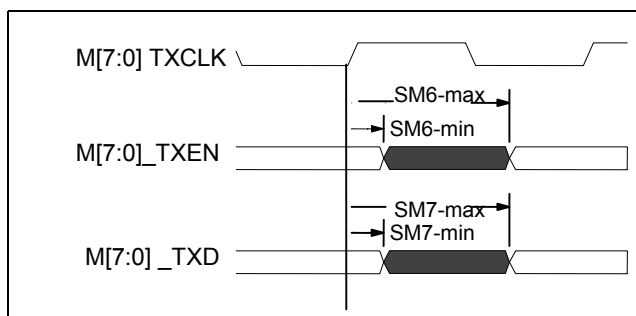
Figure 19 - AC Characteristics – General Purpose Serial Interface (TX)
