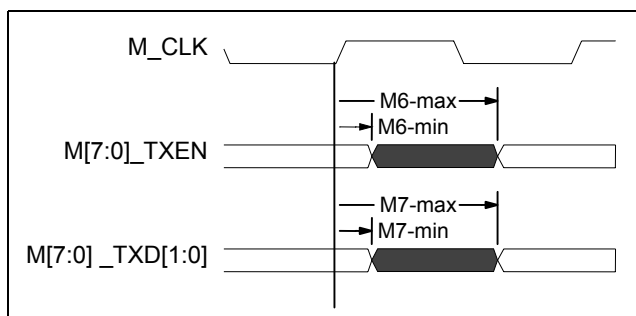
Figure 15 - AC Characteristics – Reduced media independent Interface (TX)
