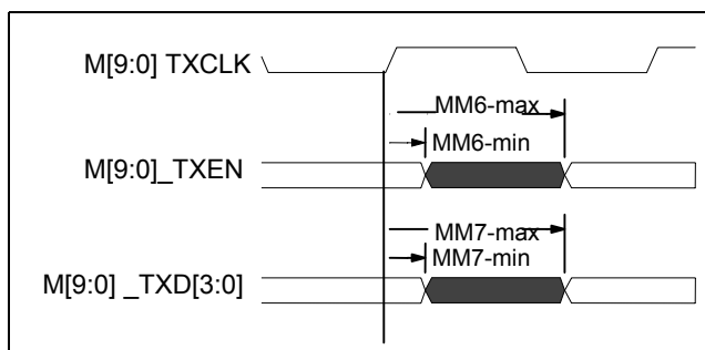
Figure 17 - AC Characteristics – Media independent Interface (TX)
