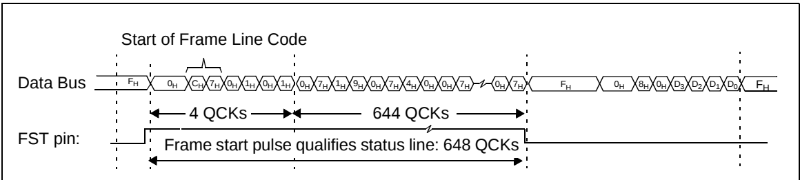
Figure 13: Detailed FST timing
