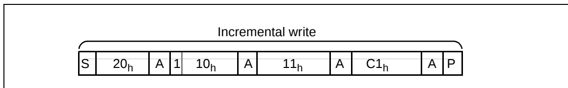
Figure 28: Multiple location write
