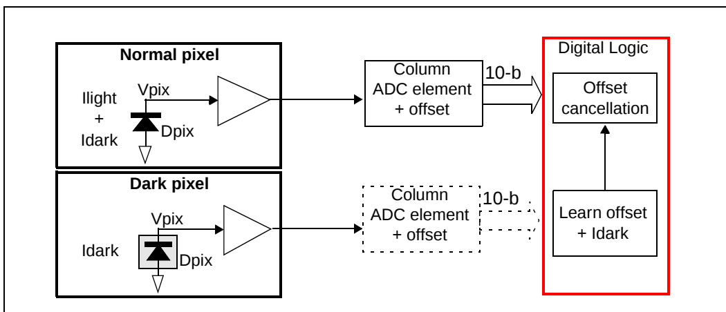
Figure 15: Overview of dark offset cancellation
