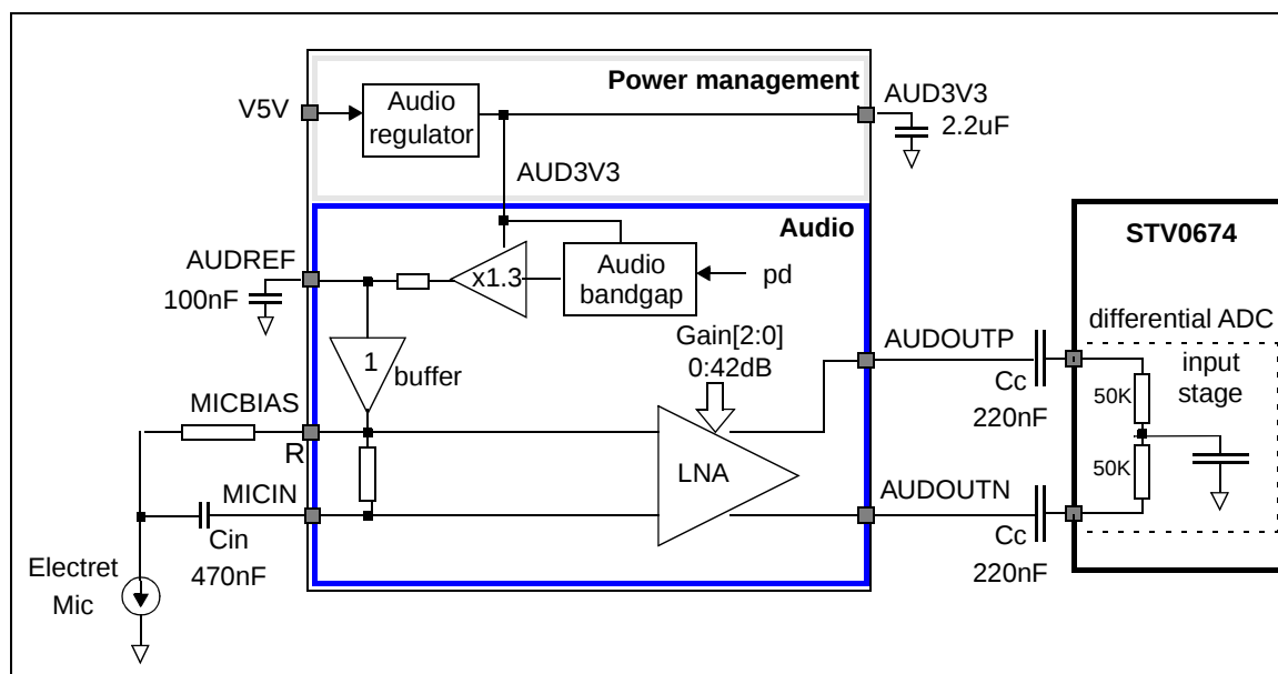
Figure 18: VV6501 audio amplifier in typical application
