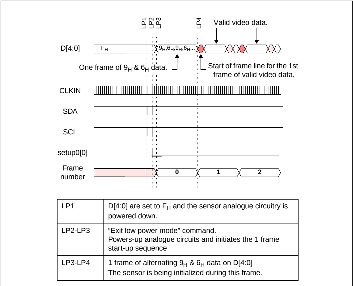
Figure 21: Exiting low-power mode
