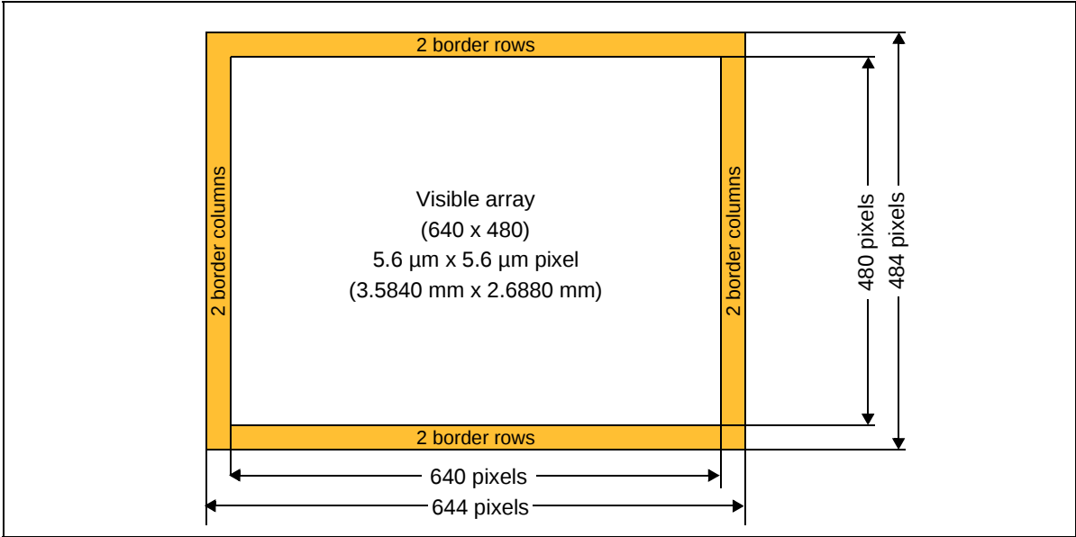
Figure 5: Pixel array
