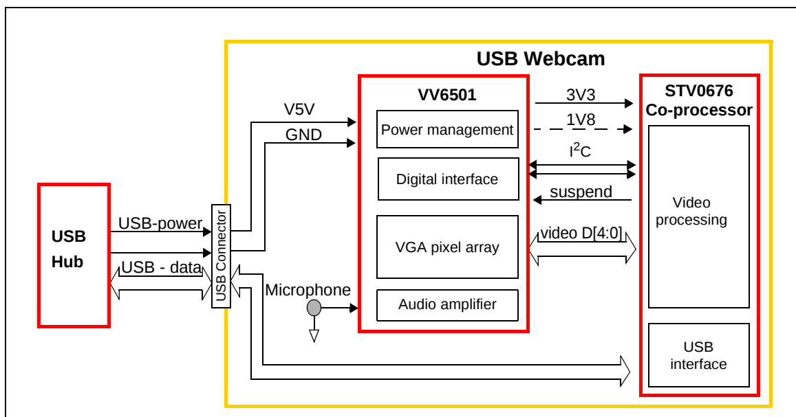
Figure 2: USB camera system using STV0676
