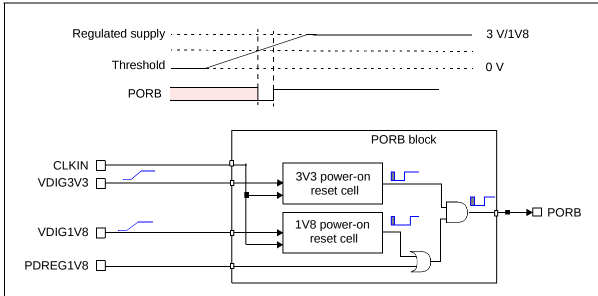
Figure 20: Power-on reset block
