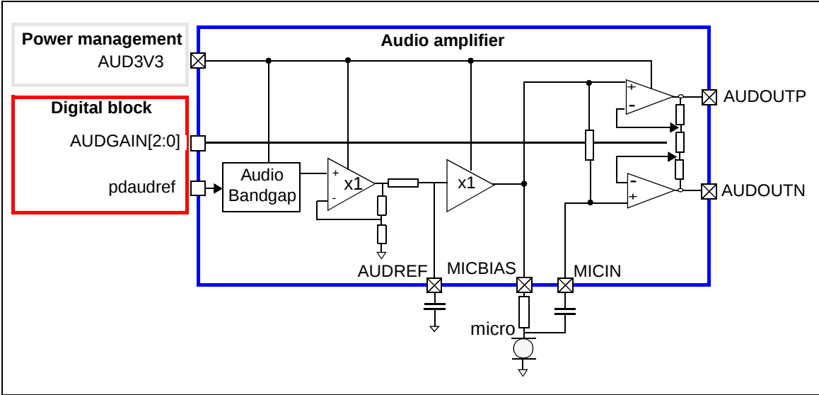
Figure 17: VV6501 audio amplifier overview
