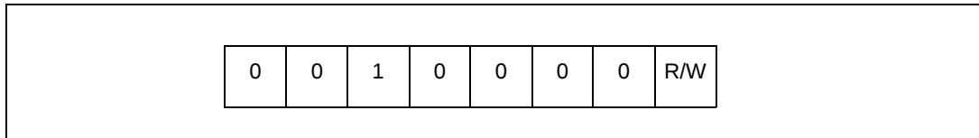
Figure 23: VV6501 Serial interface address
