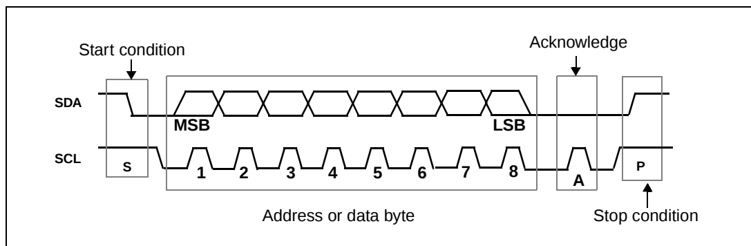
Figure 22: Serial Interface data transfer protocol
