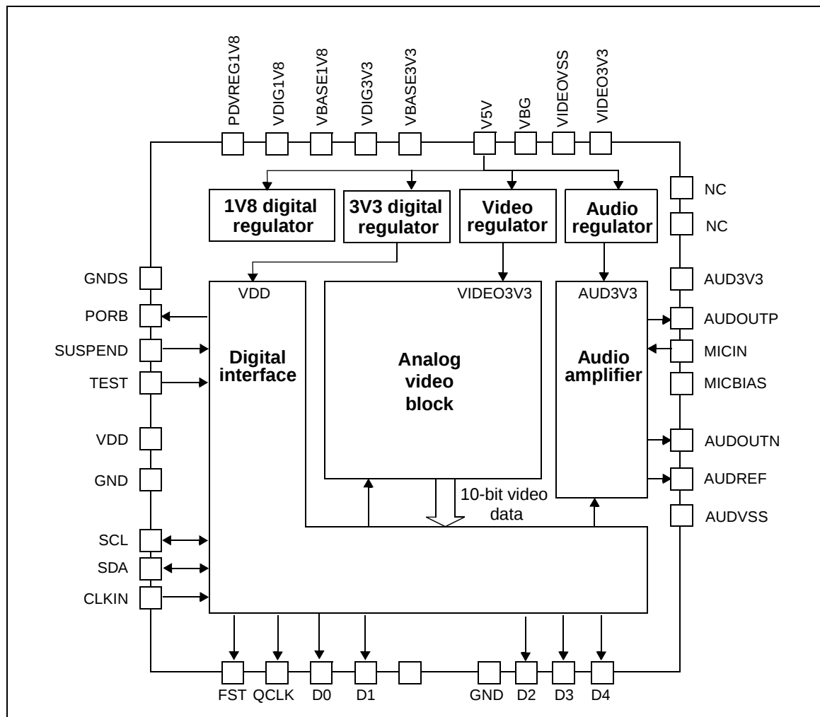
Figure 1: VV6501 block diagram
