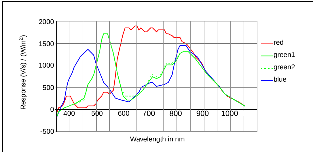
Figure 29: Spectral response
