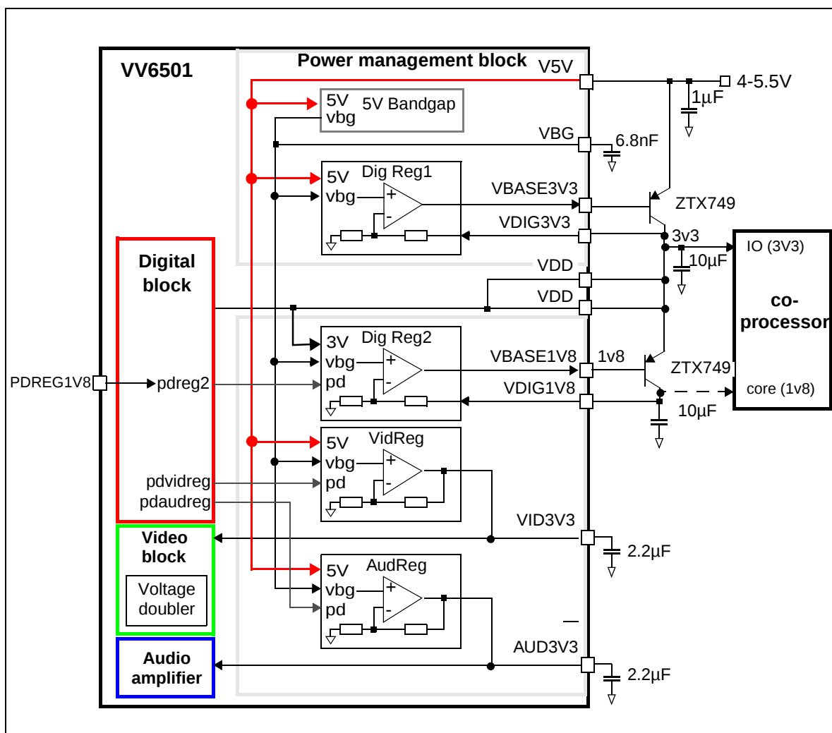
Figure 19: Voltage regulator block diagram
