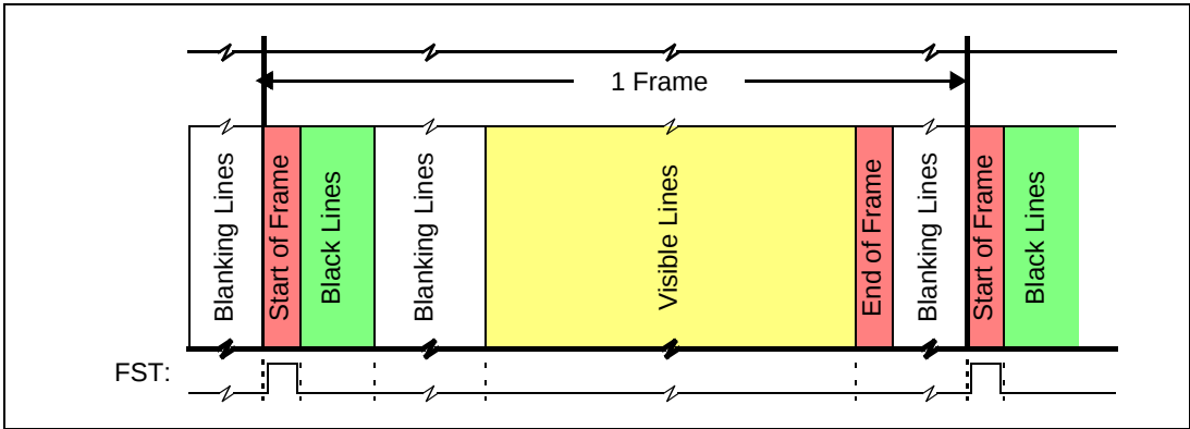
Figure 12: FST timing overview
