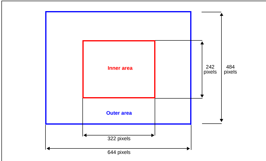
Figure 30: VV6501 array
