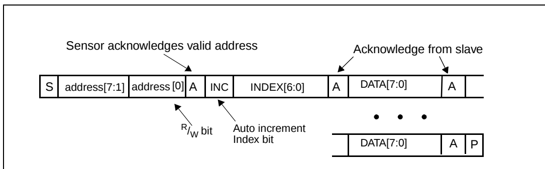
Figure 24: Serial interface data format
