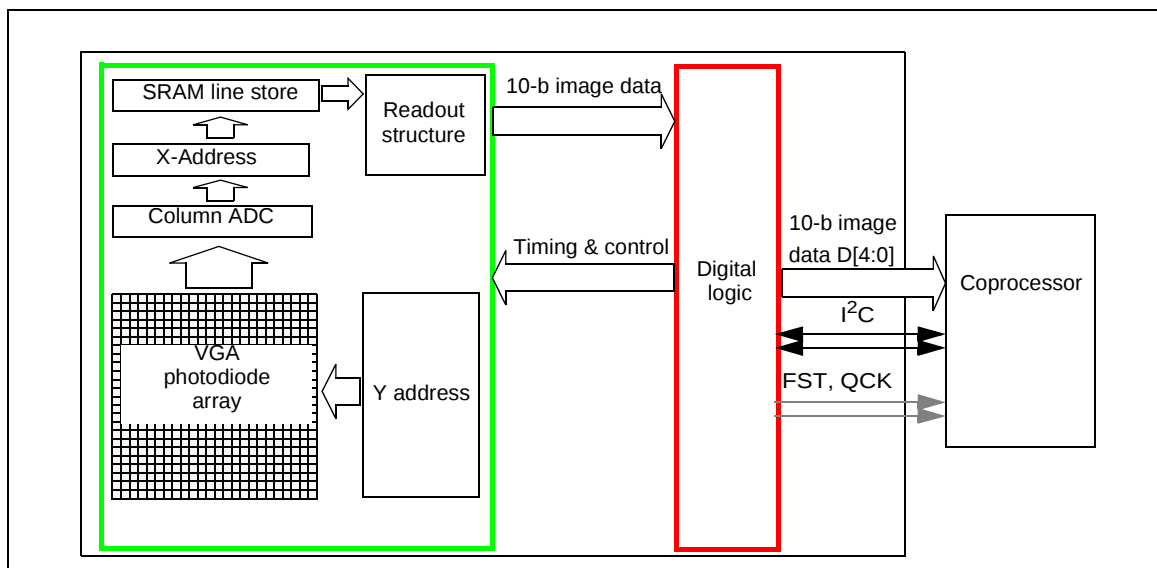
Figure 4: Overview of video block
