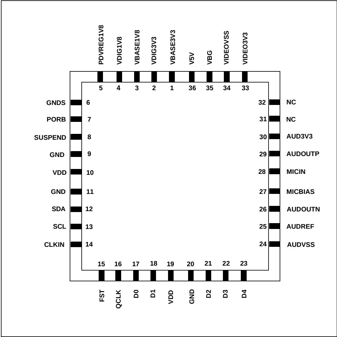
Figure 3: Pin position
