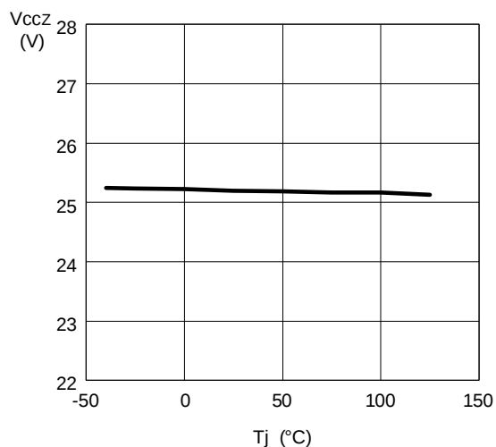
Figure 4. V CC Zener voltage vs. T j
