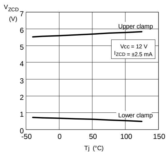
Figure 13. ZCD clamp levels vs. T_j
