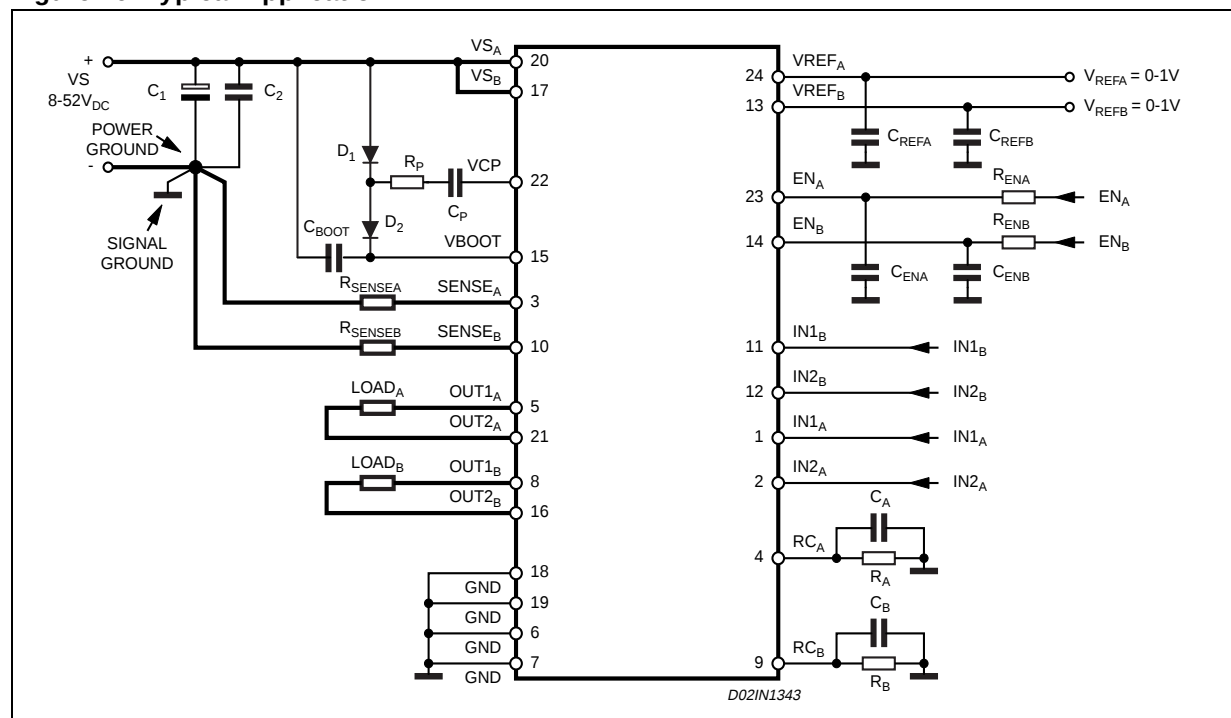
Figure 16. Typical Application
