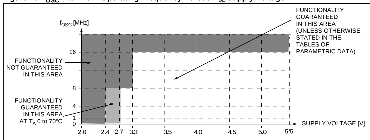
Figure 46. f_{OSC} Maximum Operating Frequency Versus V_{DD} Supply Voltage
