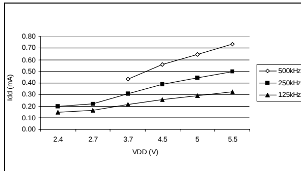
Figure 55. Typical I_{DD} in SLOW vs. f_{CPU}
