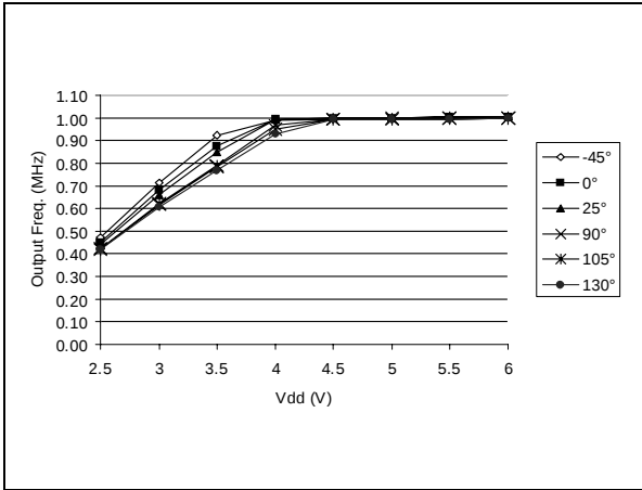
Figure 48. RC Osc Freq vs V_{DD} (Calibrated with RCCR0: 5V @ 25^{\circ}\text{C} )
