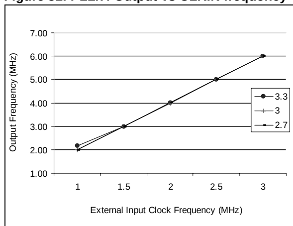
Figure 52. PLLx4 Output vs CLKIN frequency
