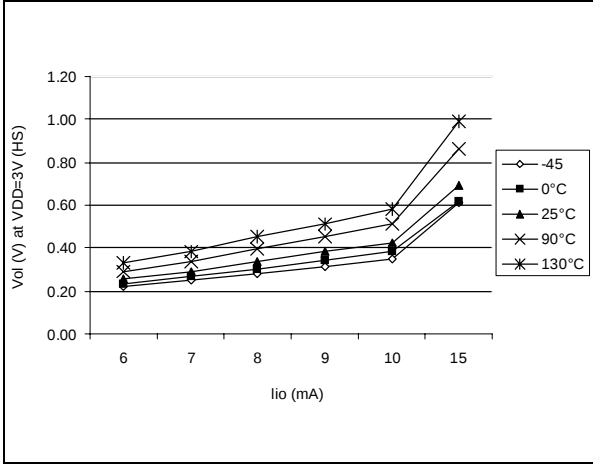
Figure 72. Typical V_{OL} at V_{DD}=3V (high-sink)
