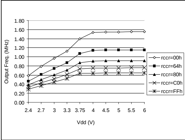
Figure 50. RC Osc Freq vs V_{DD} and RCCR Value
