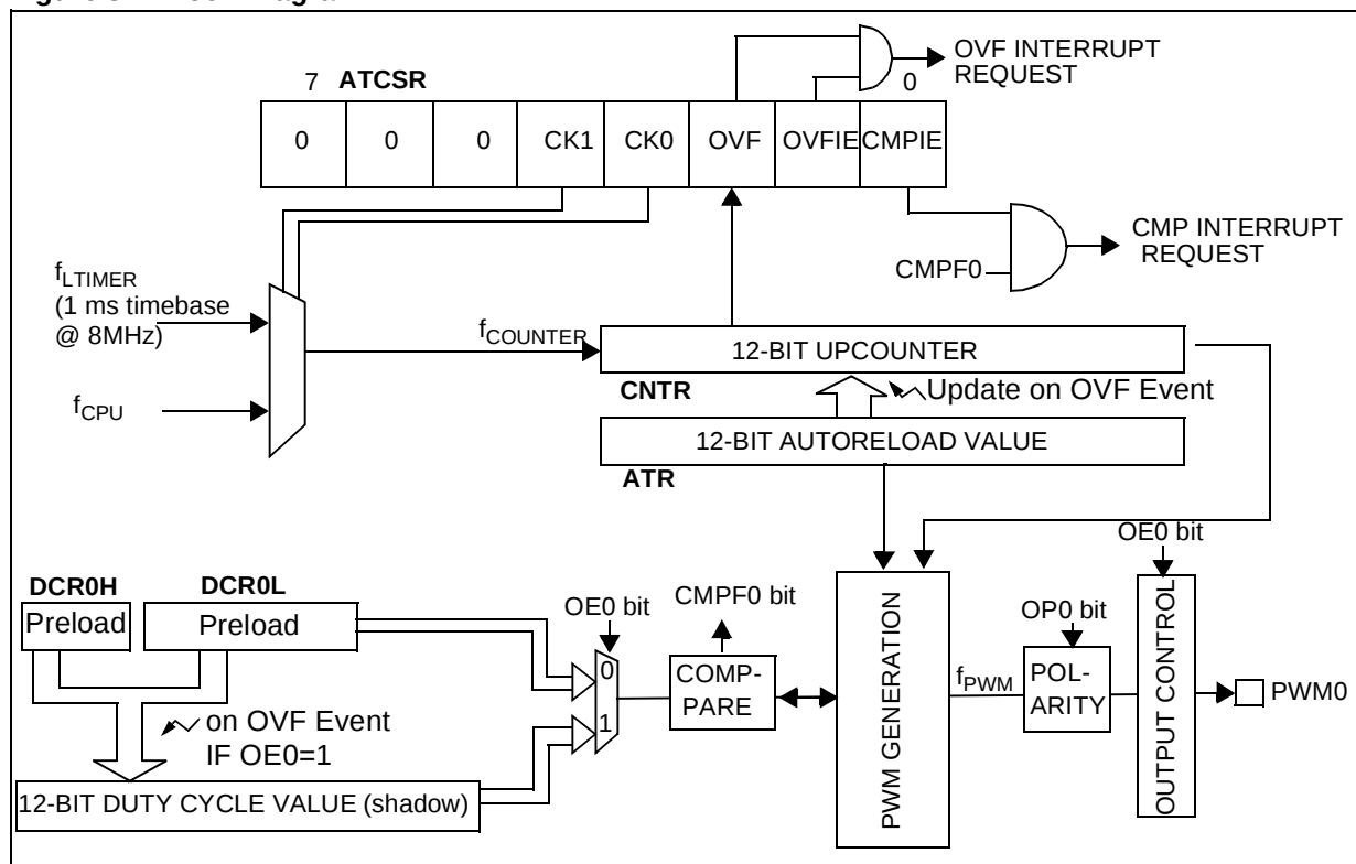
Figure 32. Block Diagram
