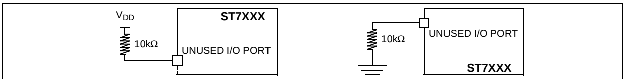
Figure 82. Two typical Applications with unused I/O Pin
