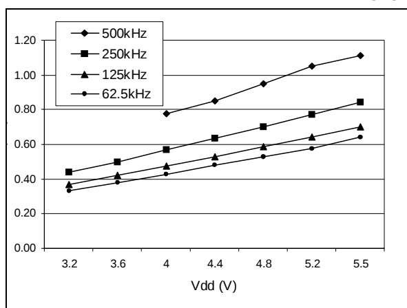
Figure 66. Typical I_{DD} in SLOW-WAIT vs. f_{CPU}
