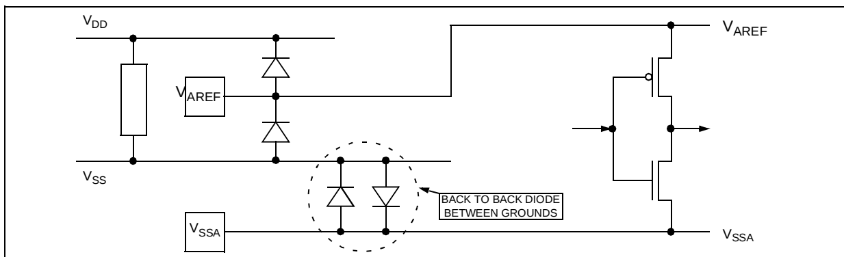
Figure 79. Multisupply Configuration
