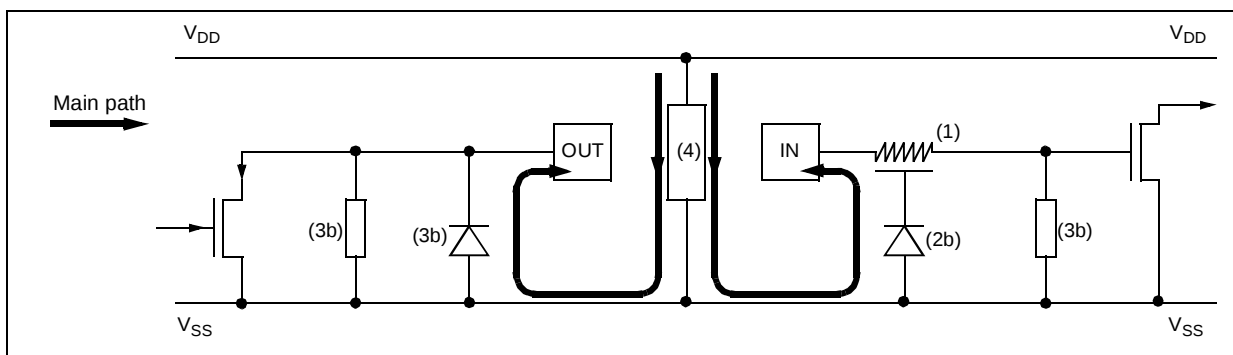
Figure 79. Multisupply Configuration
