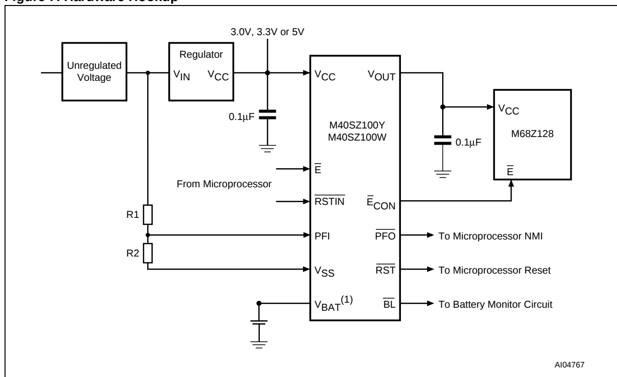
Figure 7. Hardware Hookup
