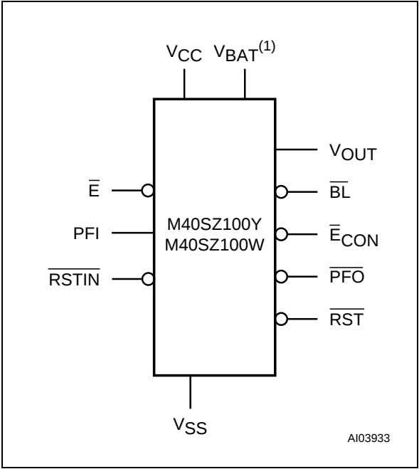
Figure 3. Logic Diagram
