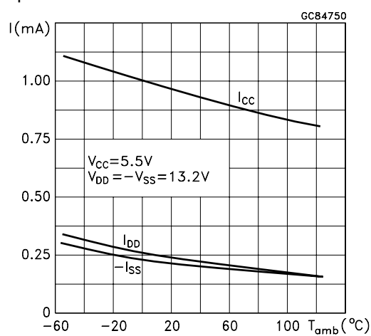
Figure 12 : Device Supply Current vs Temperature
