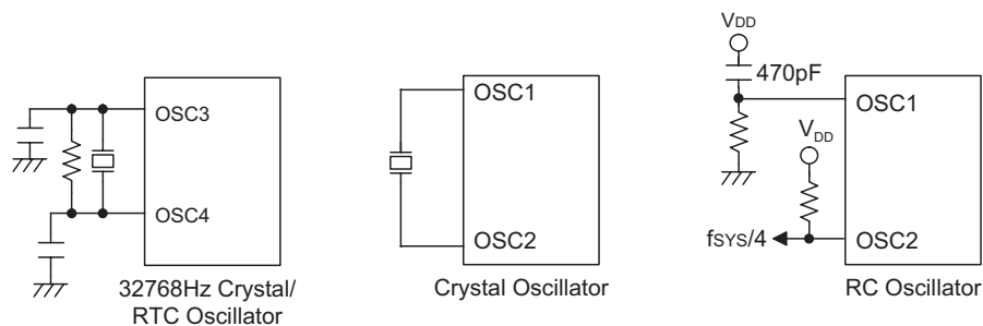
System Oscillator
