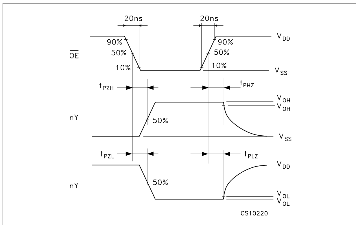
WAVEFORM 2 : PROPAGATION DELAY TIMES ( f=1\text{MHz} ; 50% duty cycle)
