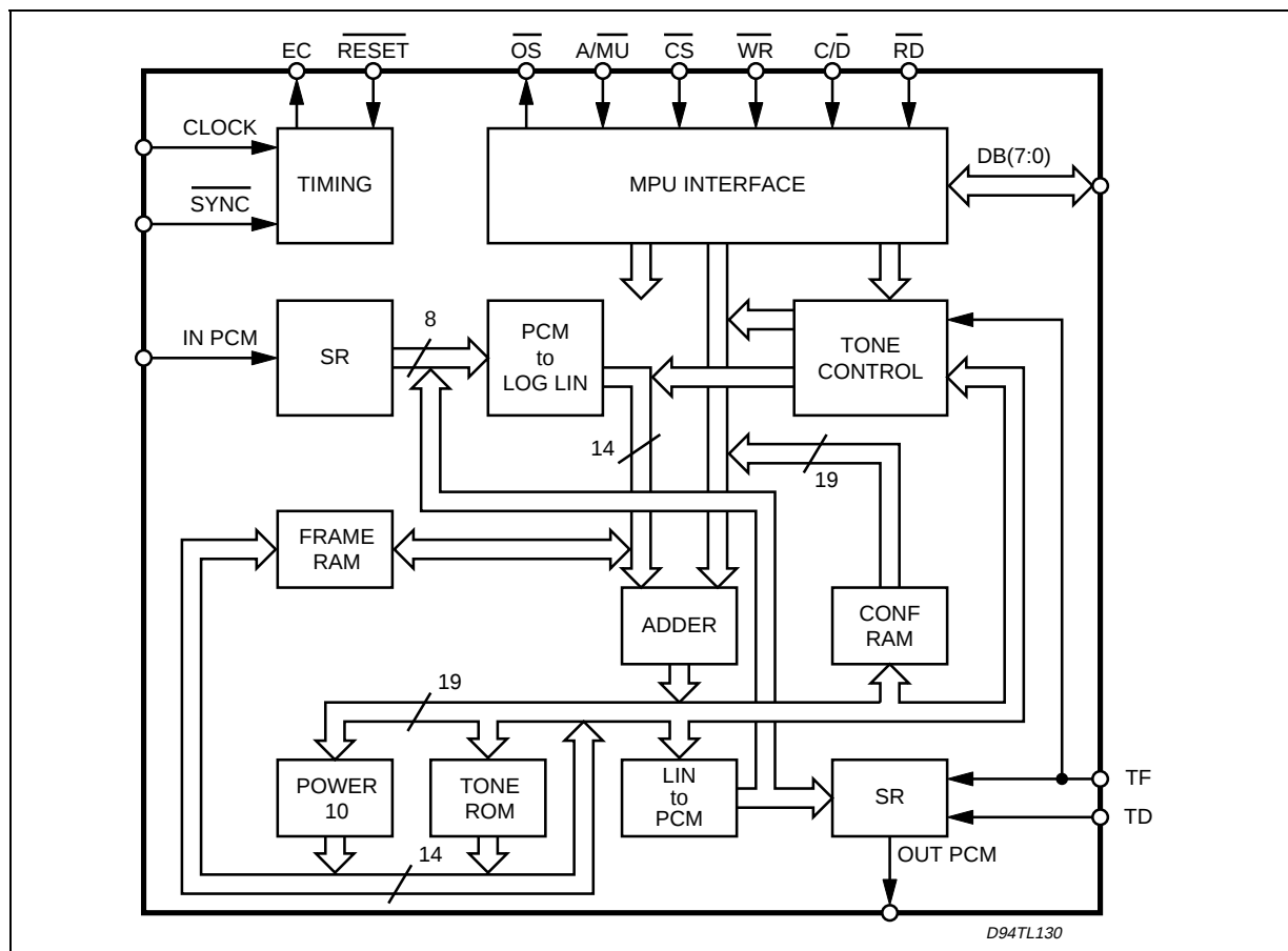
Figure 3: Block Diagram
